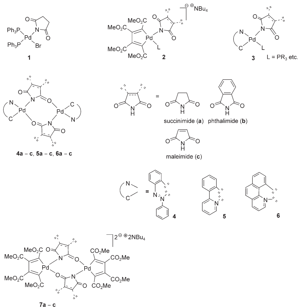
Figure 1. Neutral and anionic palladium(II) complexes containing imidate ligands.
