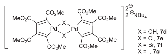
Figure 2. Anionic palladium(II) complexes containing \mu^2 -hydroxy- and \mu^2 -halide bridging ligands.
