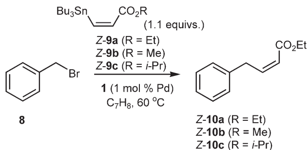
Scheme 1. Stille coupling mediated by cis -1.
