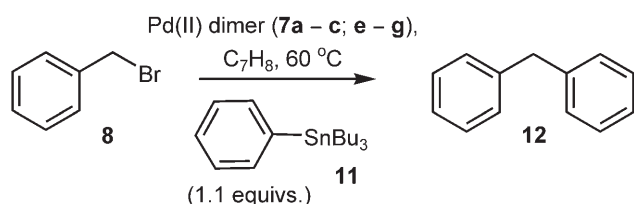
Scheme 2. Stille coupling of benzyl bromide 8 with phenylstannane 11 to give 12 .
