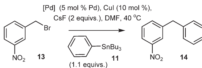
Scheme 3. Stille coupling of 3-nitrobenzyl bromide 13 with phenylstannane 11 to give 14 .
